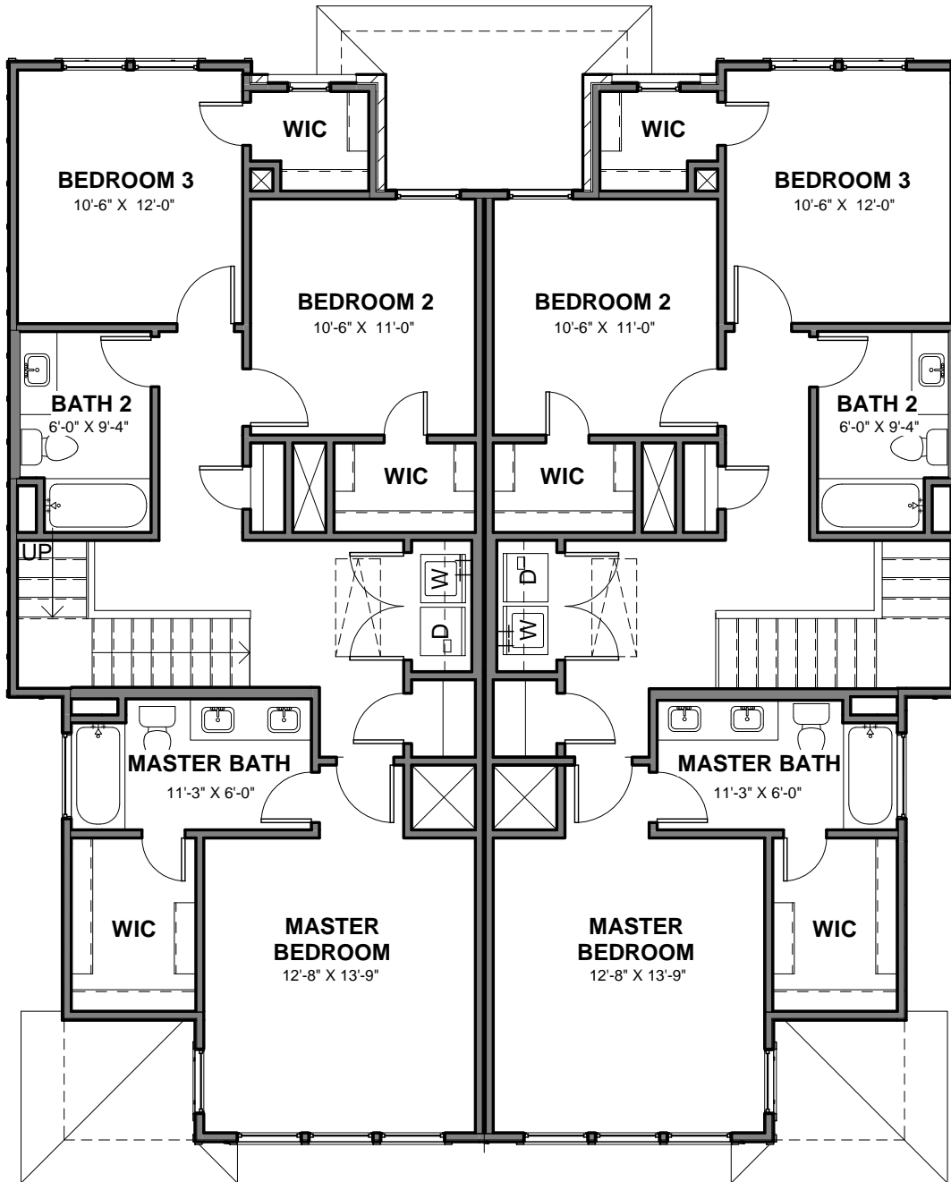
FLOOR PLAN (UPPER LEVEL) PRESENTATION
