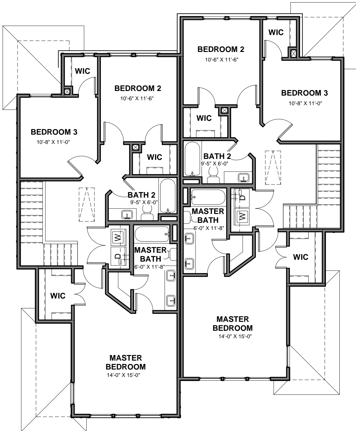
① FLOOR PLAN (UPPER LEVEL) PRES. 1/8" = 1'-0"
