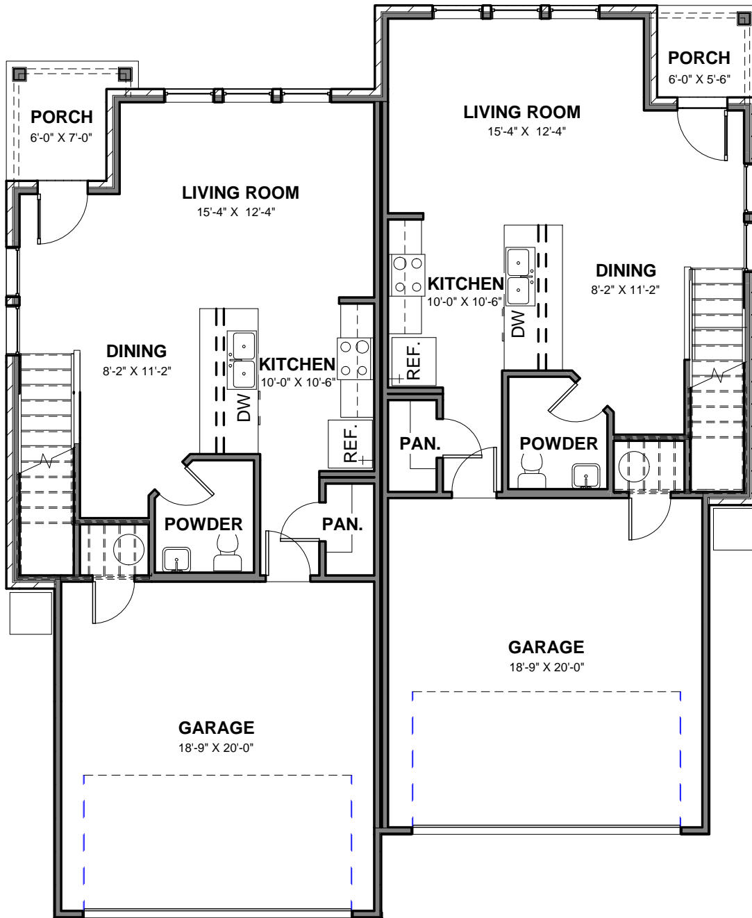
2 FLOOR PLAN (MAIN LEVEL) PRES. 1/8" = 1'-0"
